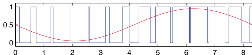
1 Phase Modulator
