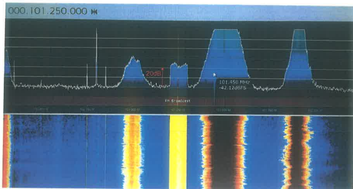
SDRSharp with RTL Dongle and small whip antenna at critical indoor location: SNR>20dB.
