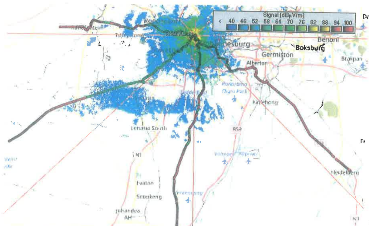
Drive-by mobile measurements at 16 QAM and 1/3 FEC against coverage prediction at 99% location probability and a threshold of 40 dBμV/m
