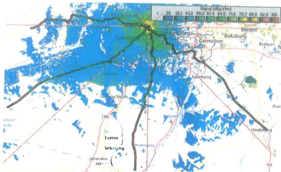
Drive-by mobile measurements at 4QAM and 1/3 FEC against coverage prediction at 99% location probability and a threshold of 29 dBμV/m
